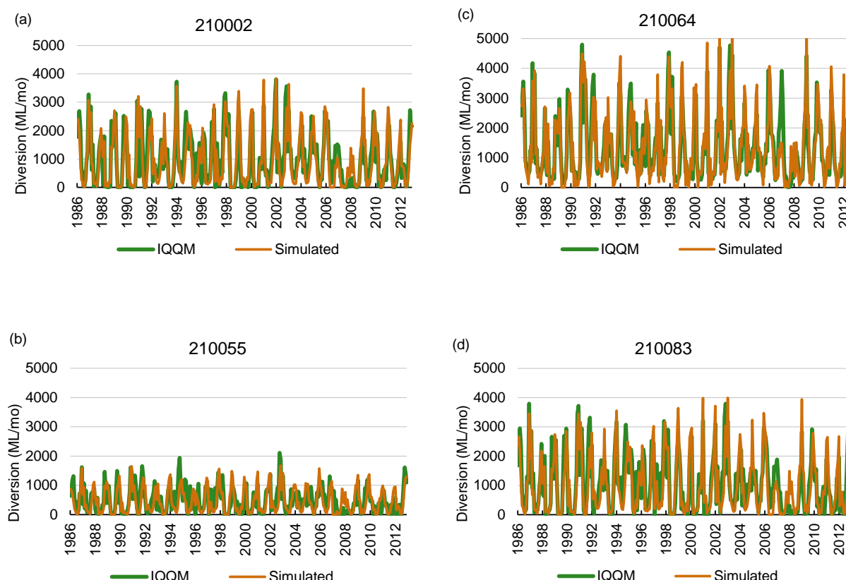
Figure 15 Example of IQQM and simulated monthly irrigation diversions for four reaches in the Hunter River
