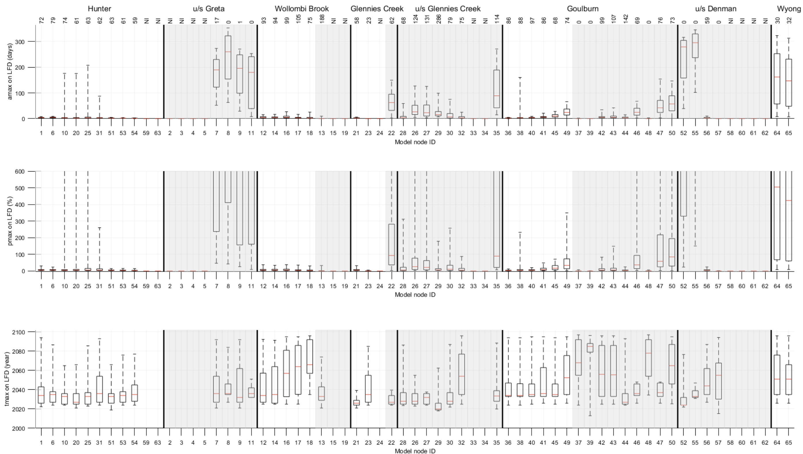
Figure 25 Hydrological changes due to the additional coal resource development on the number of low-flow days (LFD) at the 65 model nodes within the Hunter subregion
