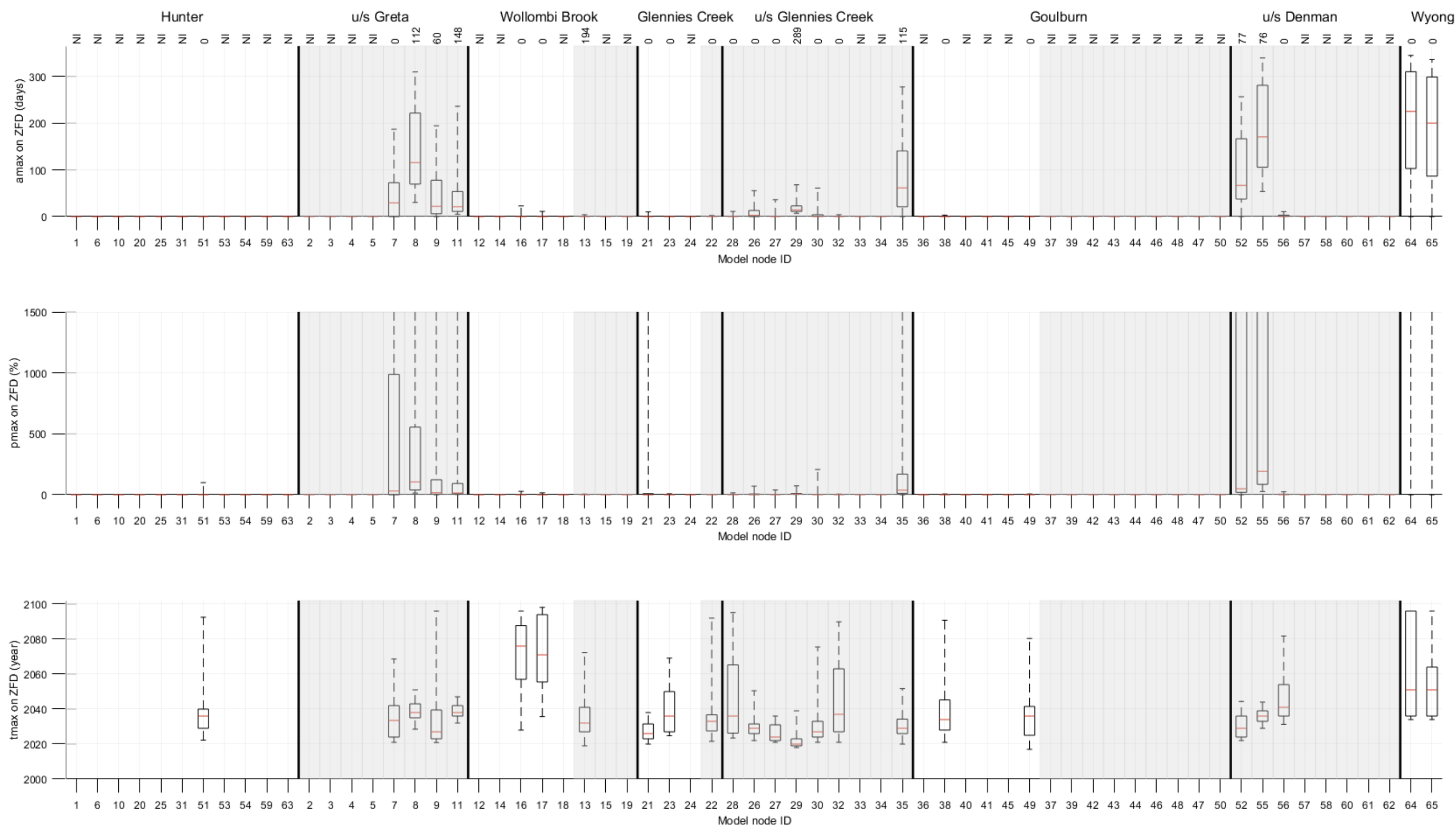
Figure 24 Hydrological changes due to the additional coal resource development on the number of zero-flow days (ZFD) at the 65 model nodes within the Hunter subregion
