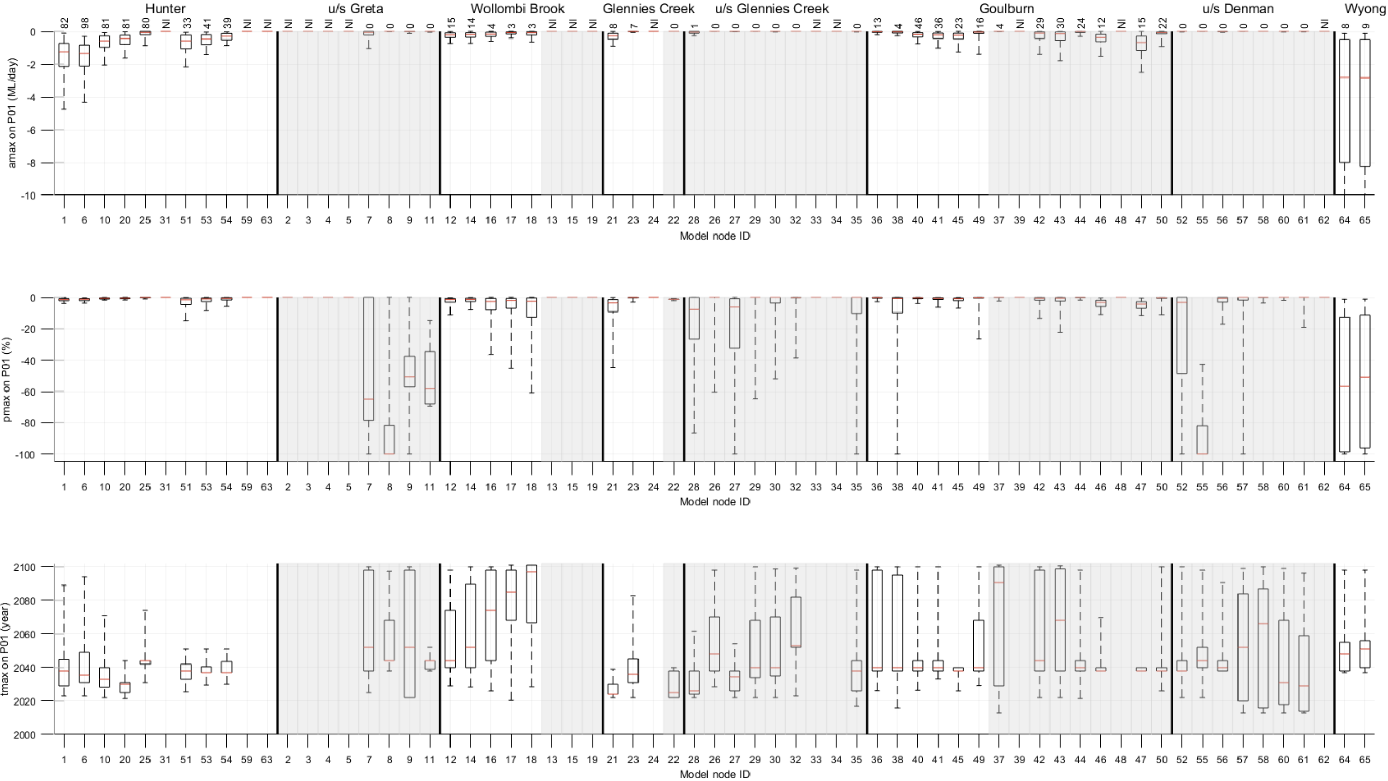
Figure 23 Hydrological changes due to additional coal resource development on daily streamflow at the 1st percentile (P01) at the 65 model nodes within the Hunter subregion
