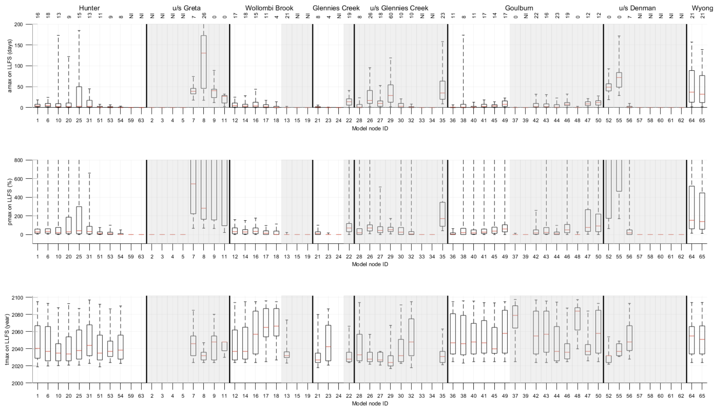
Figure 27 Hydrological changes due to the additional coal resource development on the length of longest low-flow spell (LLFS) at the 65 model nodes within the Hunter subregion
