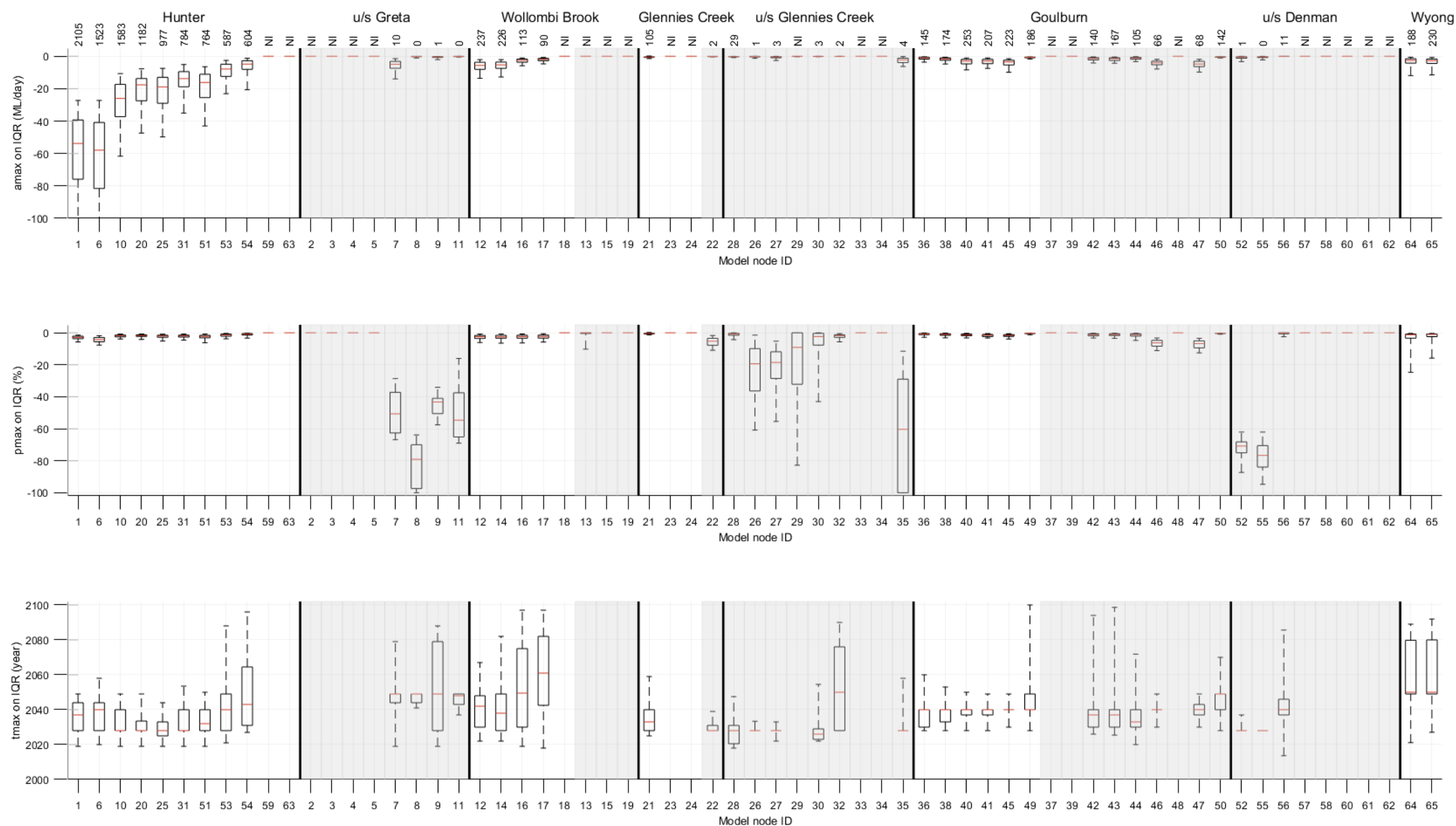
Figure 21 Hydrological changes due to additional coal resource development on interquartile range (IQR) at the 65 model nodes within the Hunter subregion
