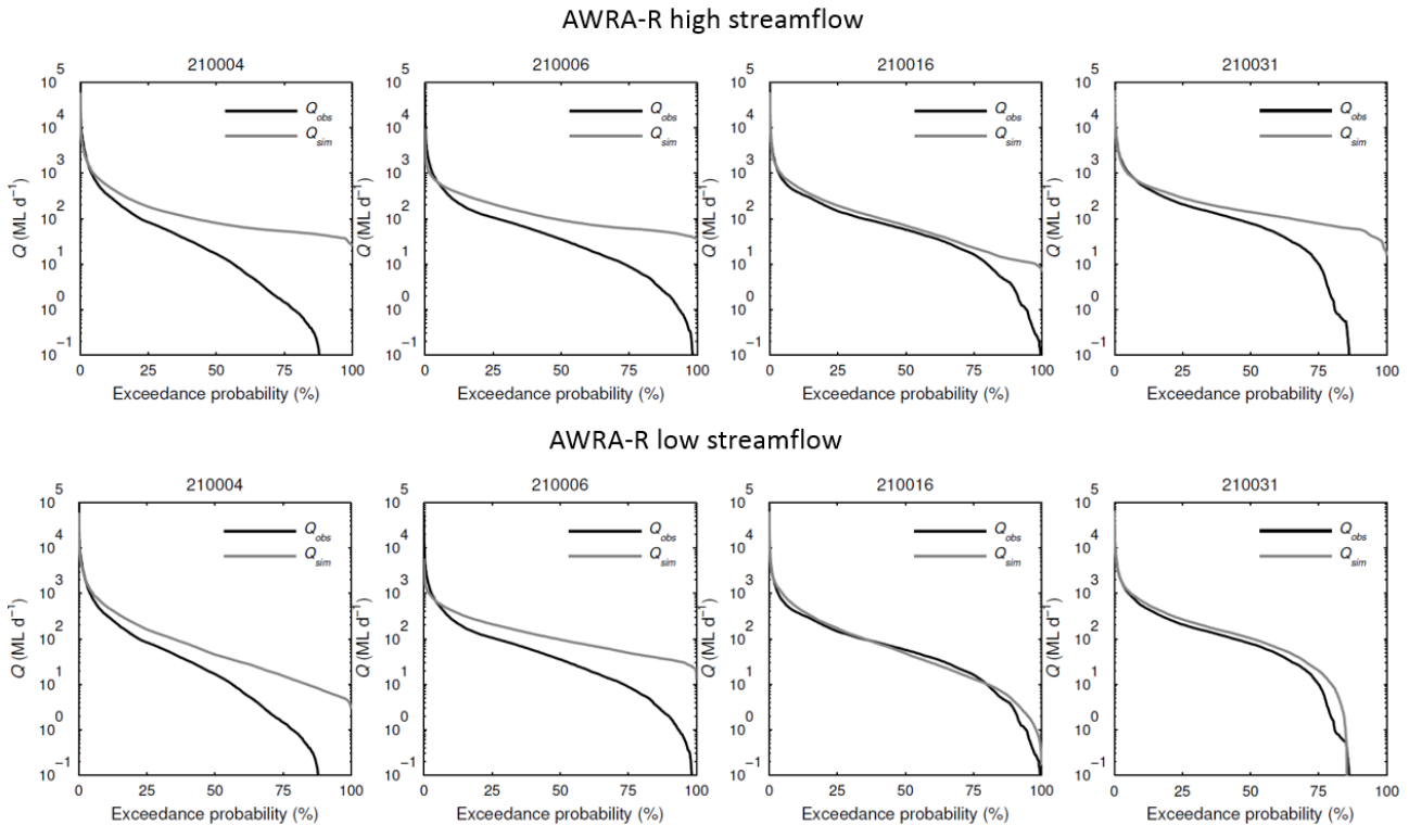
Figure 13 Flow duration curves for selected stations in Wollombi Brook (210004) and Goulburn River (210006, 210016, 210031) for AWRA-R high-streamflow calibration (top row) and AWRA-R low-streamflow calibration (bottom row), respectively
