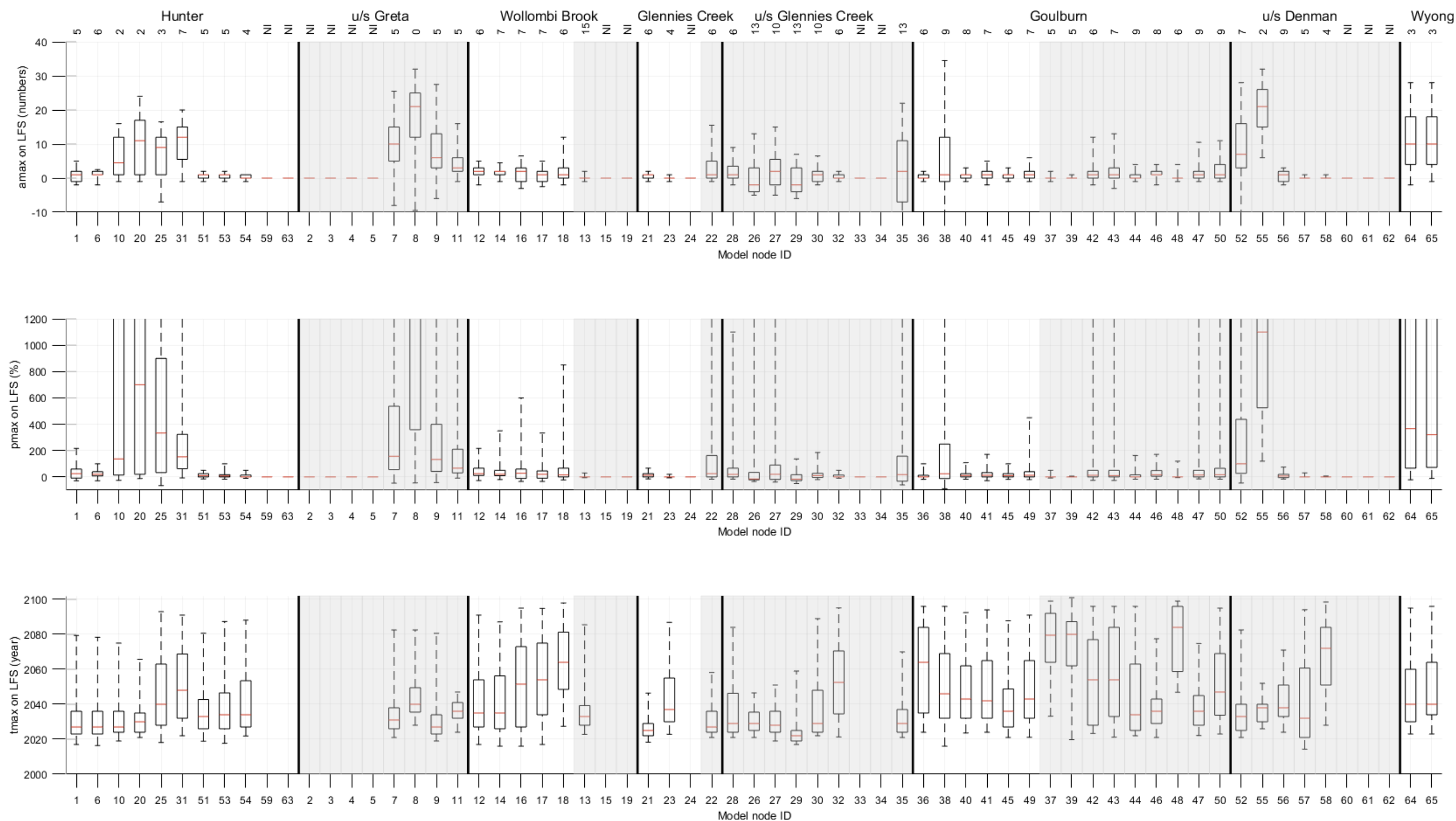
Figure 26 Hydrological changes due to the additional coal resource development on the number of low-flow spells (LFS) at the 65 model nodes within the Hunter subregion
