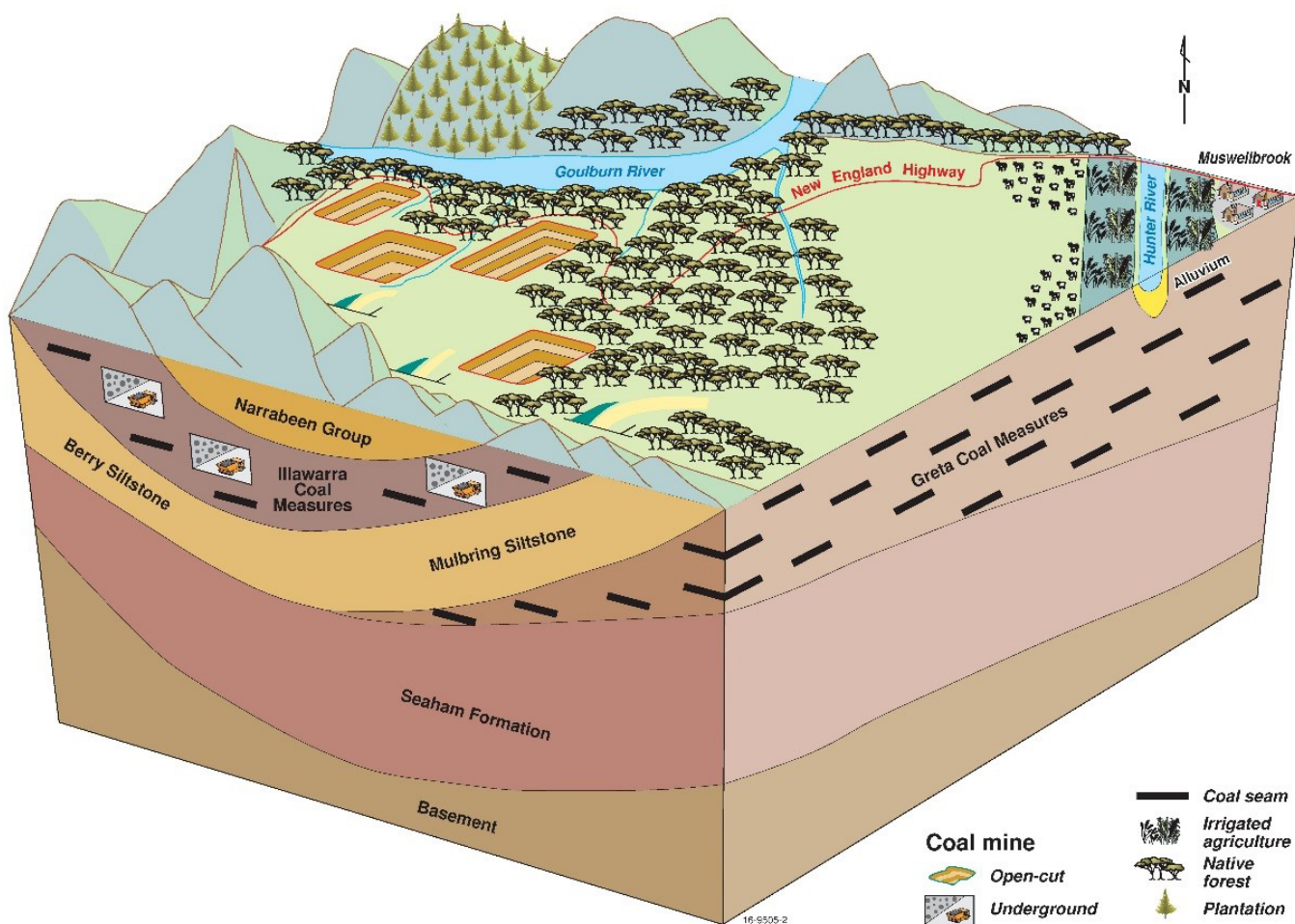
Figure 4 Regional geological model representing the Western Coalfield (west) to Hunter coalfield (east) in the Goulburn river basin in the west of the subregion
