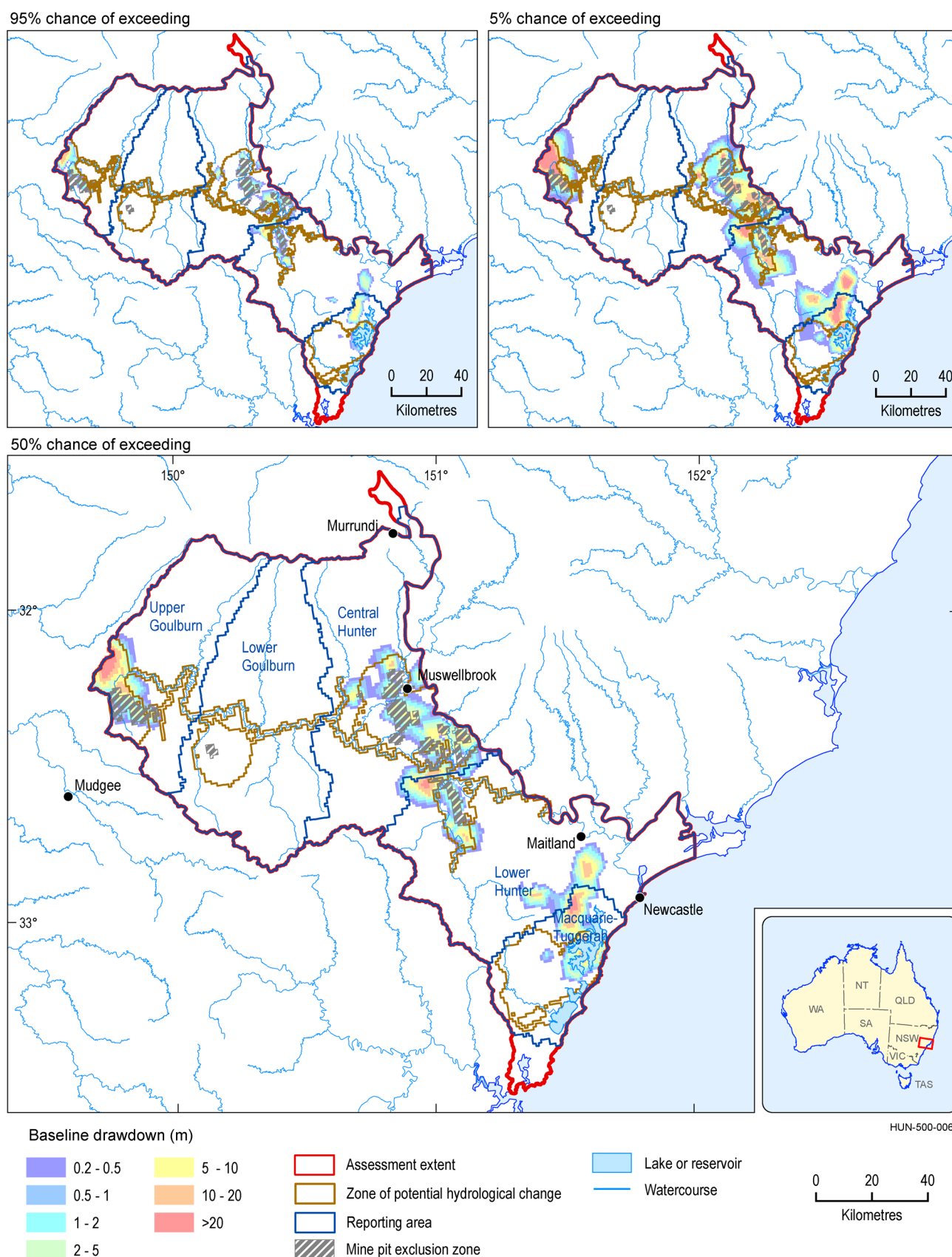
Figure 9 Baseline drawdown (m) in the regional watertable (95%, 50% and 5% chance of exceeding given values of drawdown)
