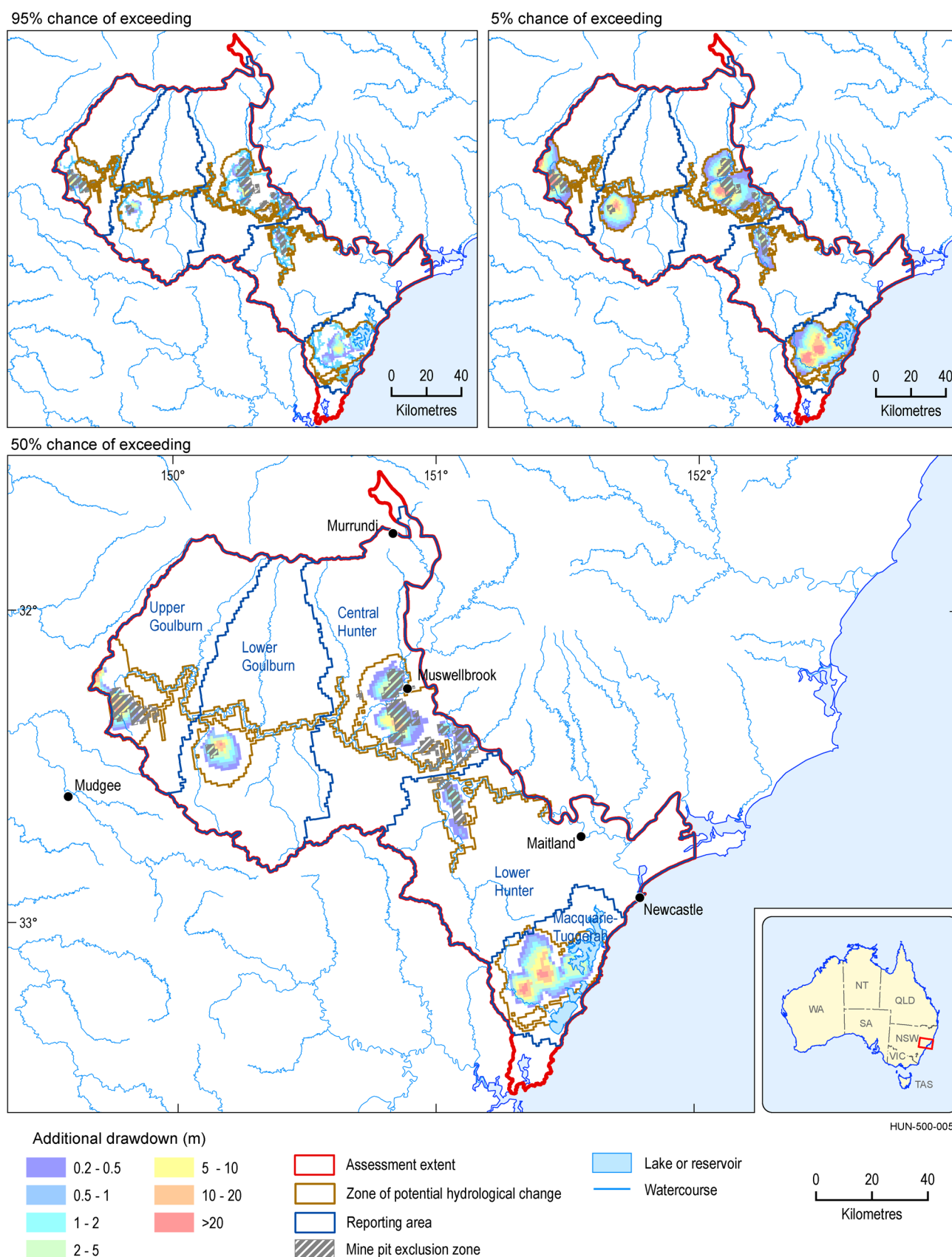
Figure 8 Additional drawdown (m) in the regional watertable (95%, 50% and 5% chance of exceeding given values of drawdown)
