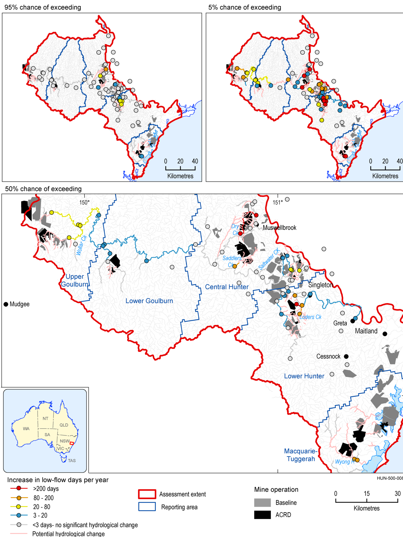
Figure 12 Maximum increase in the number of low-flow days due to additional coal resource development (95%, 50% and 5% chance of exceeding given values of change)
